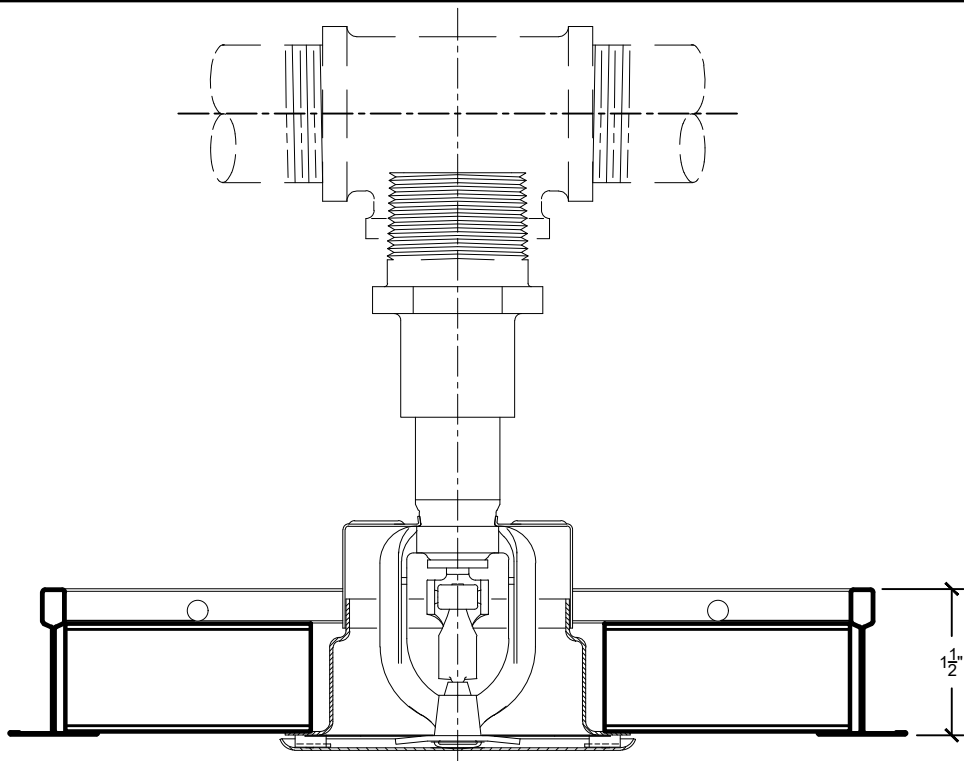
LAY IN PANEL SPRINKLER PENETRATION
