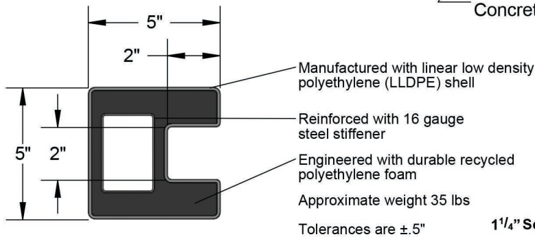
End Post Cutaway
