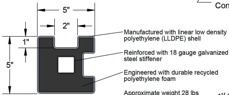
Corner Post Cutaway
