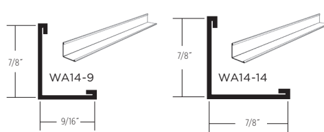
WALL ANGLE
