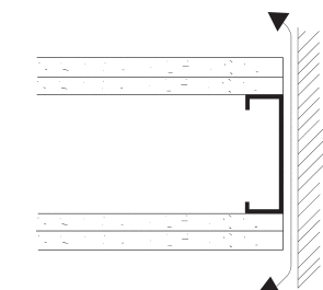
Plan Metal Stud Around Flanking Partition Ends
