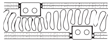
Plan Indicating Caulking of Openings Through Partitions
