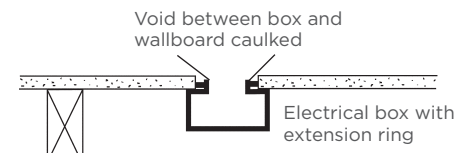
Plan Outlet Box Detail
