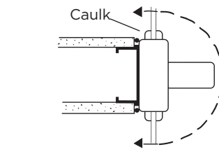
Plan Typical Partition Mullion Intersection
