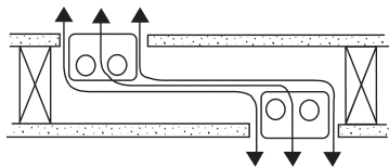
Plan Through Partitions, Openings, Outlet Boxes
